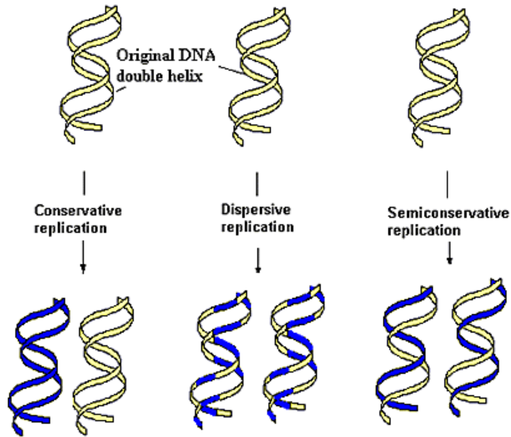
Possible Models of DNA Replication
